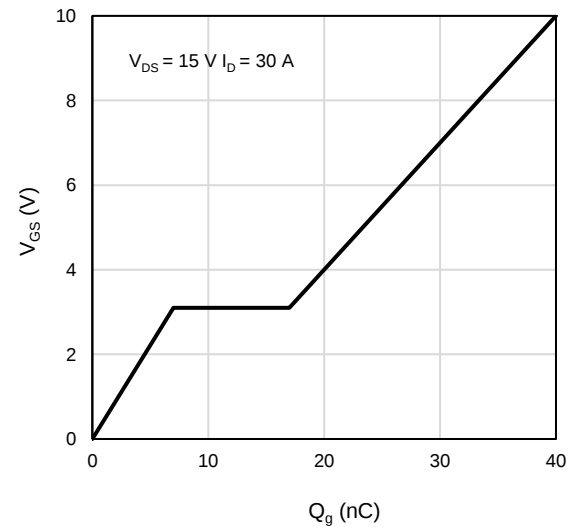
Figure 10: Gate-Charge Characteristics
