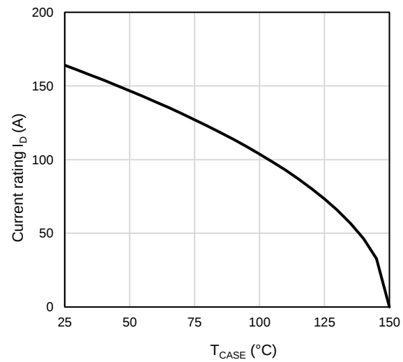
Figure 12: Current De-rating
